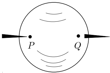
Fig. 1: Virasoro situation ( g = 0 , N = 2 )
